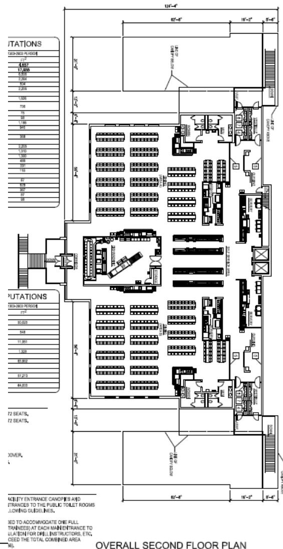
OVERALL SECOND FLOOR PLAN
